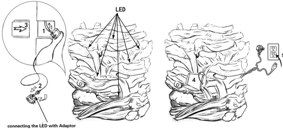
connecting the LED with Adaptor
